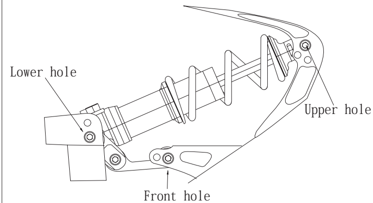
CURNUTT Shocks 6 inch wheel travel
