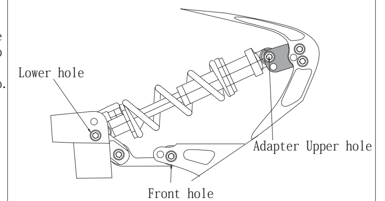
FOX Shocks 6 inch wheel travel
