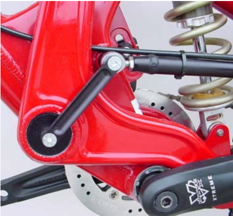
Front View of Floating Brake Rod
